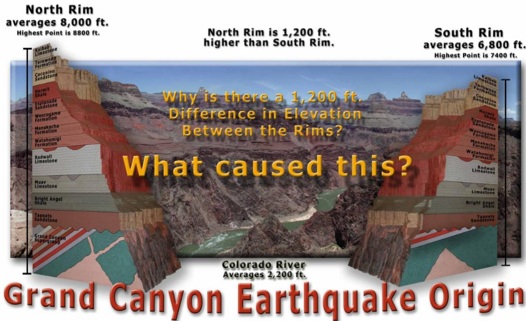
8.3.13 - The Grand Canyon Earthquake Origin diagram illustrates the 1200-foot difference in the two rims of the world's most famous canyon. Geologists have apparently overlooked the physical evidence of the Grand Canyon's origin. They have never seen an earthquake shift anywhere near the size of the shift produced by the Grand Canyon Earthquake. Grand Canyon data - http://www.nps.gov/grca/parkmgmt/statistics.htm .
