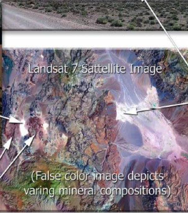
Fig 8.5.12 – In the false color Landsat satellite image of Death Valley, California, a variety of mineral deposits are apparent. Notice the two patches of white, which are Racetrack Playa Clay and Mesquite Sand Dunes. There are no 'white' mountains around them from which weathered or eroded material appears to have come. Apparently, this was overlooked by geologists, which is understandable since they had no knowledge of hydrofountains and their landscape-changing role, especially during the Flood. Fault lines run right through this area, evident by the lava extrusions in the vicinity, which testify to the earthquake friction that was generated here, which caused hydrofountains to erupt and spew clay and sand onto the surrounding surface.
