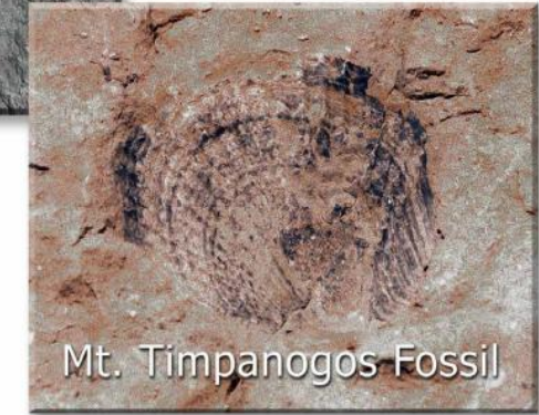
Fig 8.2.2 – Fossilized seashells are found near the summits of Mt. Timpanogos, Utah, USA and Mt. Cloudcroft, New Mexico, USA, both over 9,000 feet (2,700 meters) in elevation with no evidence they are rising. Since such fossil formations could have only formed in an ocean, it is clear that water once covered these and other mountains around the globe. The real question is how were they covered? Geologists have relied upon uniformitarianism—but this theory has failed, leaving modern geology with no real mechanism to answer this question. The Universal Flood Model finally identifies the mechanism explaining how a universal flood covered the entire surface of the Earth, including all of its mountains.
