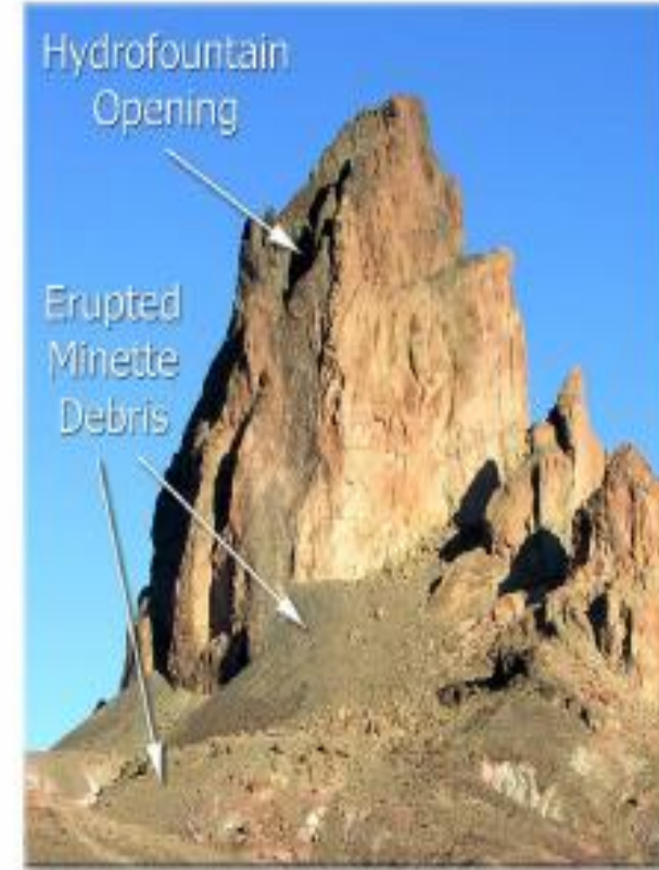
Surrounding plain has no deep valleys or riverbeds.
