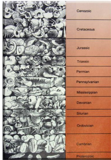
Geological Time Scale With Evolution of Life Through the Fossil Record (U. S. Geological Survey)
